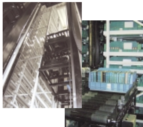
Kashiwa Library-ASRS (Automated Storage and Retrieval System)
